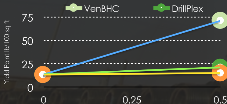
Yield Point Behavior of Ven-BHC™ vs DRILPLEX™ & MMO at 0.5 lb/bbl in 10 lb/bbl Treated (Peptized) Bentonite
